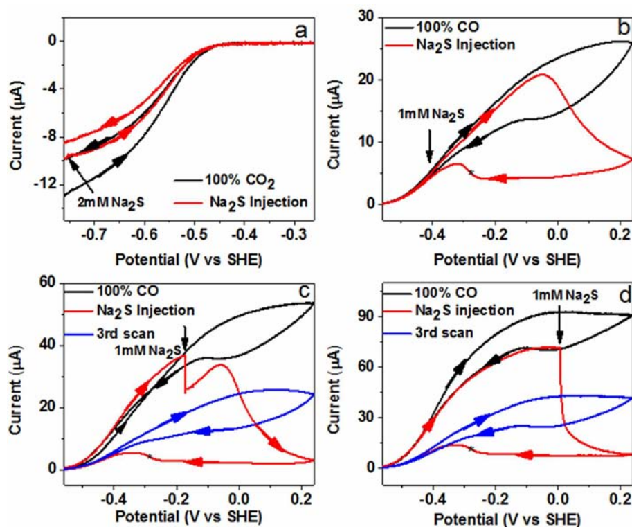
Figure 6. Potential control of CODH I_{Ch} inhibition by sulfide: 1 mM Na_2S or 2 mM Na_2S (final concentration) was injected at different potentials. The asterisk refers to the reactivation potential. Experimental conditions: 25 °C, 0.2 M MES buffer (pH 7.0), rotation rate 3500 rpm, scan rate 1 mV/s.
