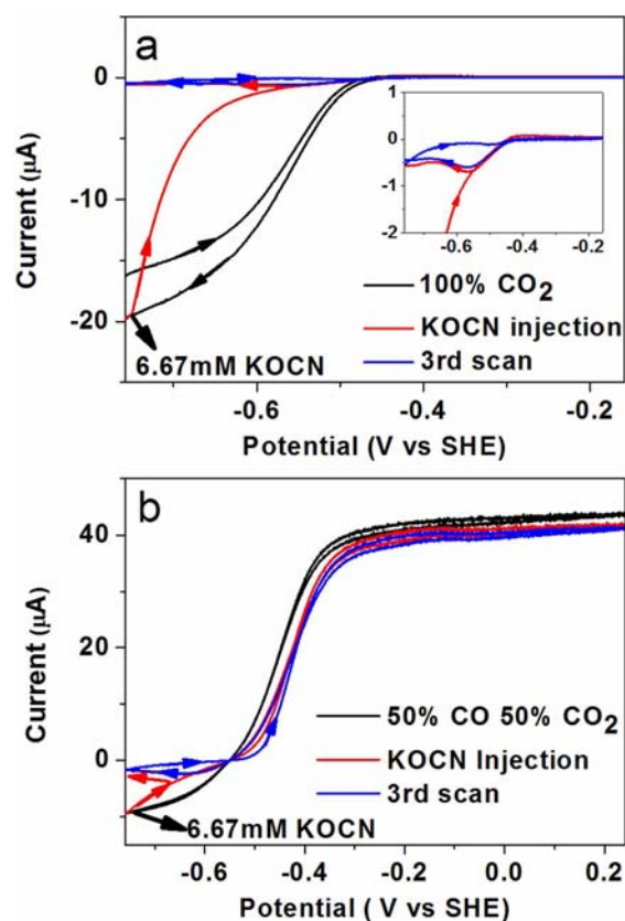
Figure 4. Inhibition of CODH I_{\text{Ch}} by cyanate. Potassium cyanate was injected (final concentration in the solution is 6.67 mM) into the electrochemical cell under a gas atmosphere of 100% \text{CO}_2 (Figure 3a) and 50% CO, 50% \text{CO}_2 (Figure 3b). Experimental conditions: 25 °C, 0.2 M MES buffer (pH 7.0), rotation rate 3500 rpm, scan rate 1 mV/s.
