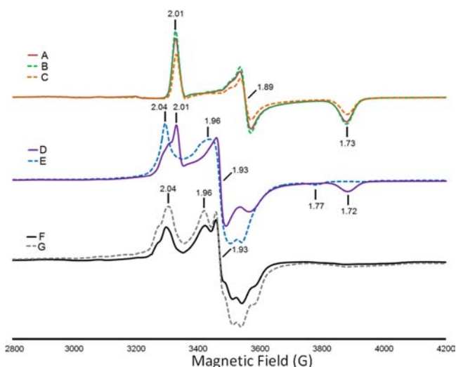
Figure 5. EPR spectra of CODH I_{Ch} (A) oxidized with benzyl viologen; (B) oxidized with benzyl viologen and in the presence of 1 mM potassium cyanate; (C) oxidized with benzyl viologen and in the presence of 20 mM potassium cyanate; (D) reduced with CO; (E) upon CO reduction, in the presence of 1 mM potassium cyanate; (F) reduced with dithionite; (G) reduced with dithionite and then in the presence of 20 mM potassium cyanate. EPR conditions: modulation amplitude 10 G for all spectra and (temperature, microwave power, frequency) (A) 12 K, 41.2 mW, 9.38 GHz; (B) 12 K, 41.18 mW, 9.38 GHz; (C) 12 K, 41.2 mW, 9.383 GHz; (D) 10 K, 41.22 mW, 9.382 GHz; (E) 12 K, 41.21 mW, 9.379 GHz; (F) 12 K, 41.21 mW, 9.38 GHz; (G) 11 K, 41.21 mW, 9.381 GHz.
