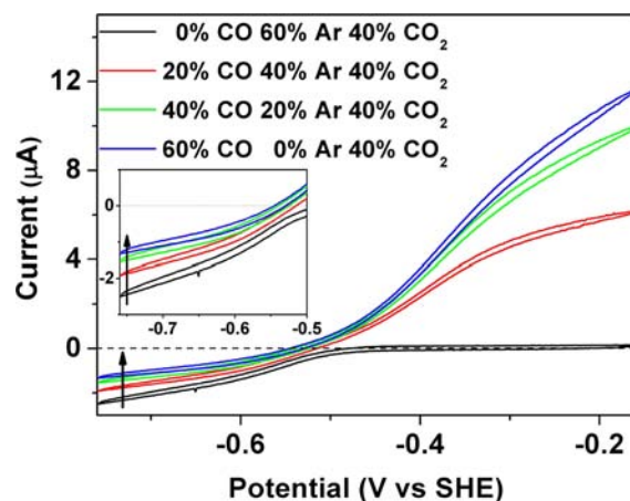
Figure 2. Inhibition of CODH I_{Ch} by CO. Different partial pressures of CO were introduced into the electrochemical cell to measure product inhibition. As the CO concentration increases, the electrocatalytic current for CO 2 reduction decreases. The inset enlarges the region in which CO 2 reduction occurs. Experimental conditions: 25 °C, 0.2 M MES buffer (pH 7.0), rotation rate 3500 rpm, scan rate 10 mV/s.
